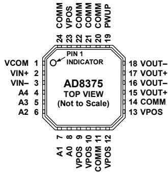
Figure 3. 24-Lead LFCSP
